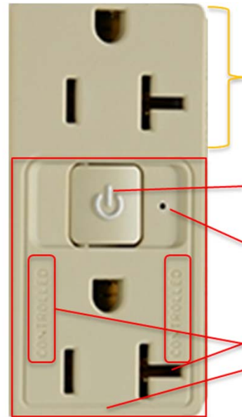
Half Controlled RF receptacle
