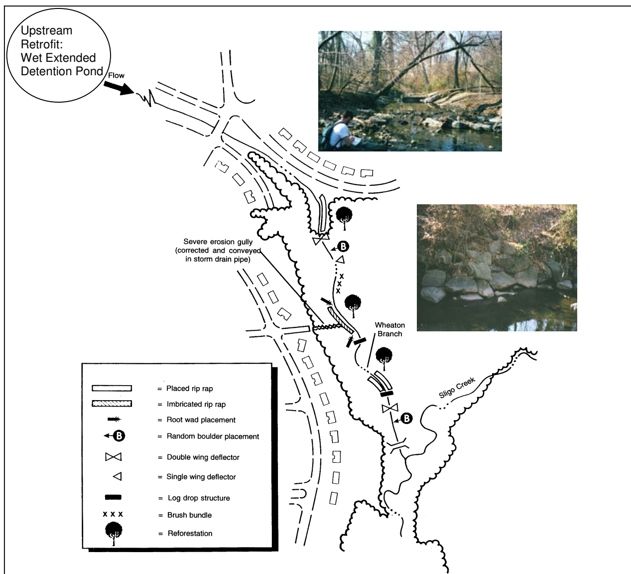
Figure 21: Example of Comprehensive Stream Restoration Approach
