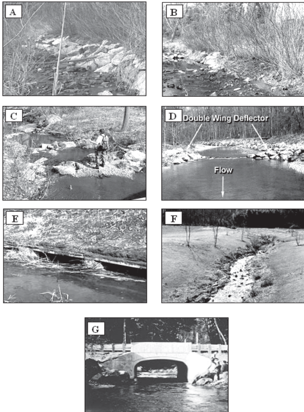
Figure 20: The Seven Basic Types of Stream Repair Techniques
