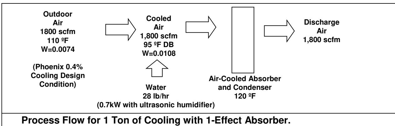
Figure 19: Intermittent Evaporative Cooling
