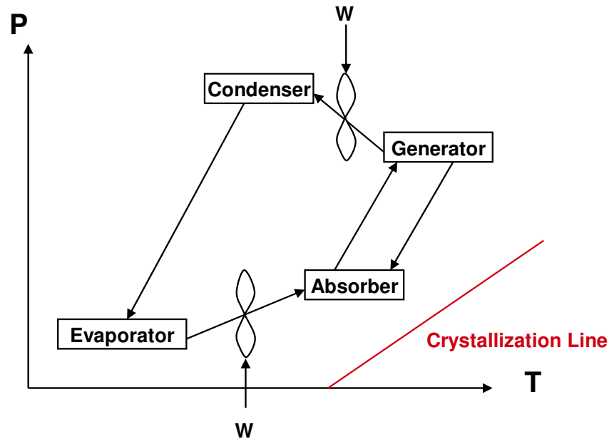
Figure 18: Dropping Generator Pressure (Shown Combined with Boosting Absorber Pressure)
