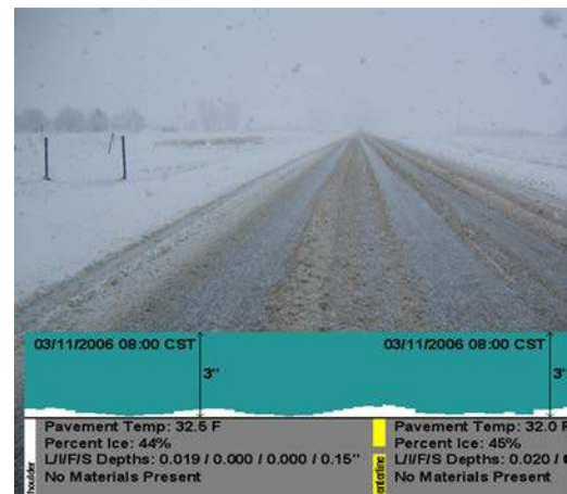
Figure SD-1. Surface conditions predicted by MDSS closely match actual road conditions.
