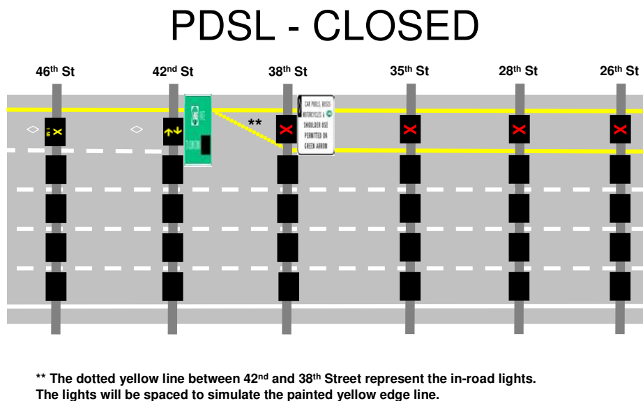
Figure MN-6. Striping and signing with PDSL closed.
