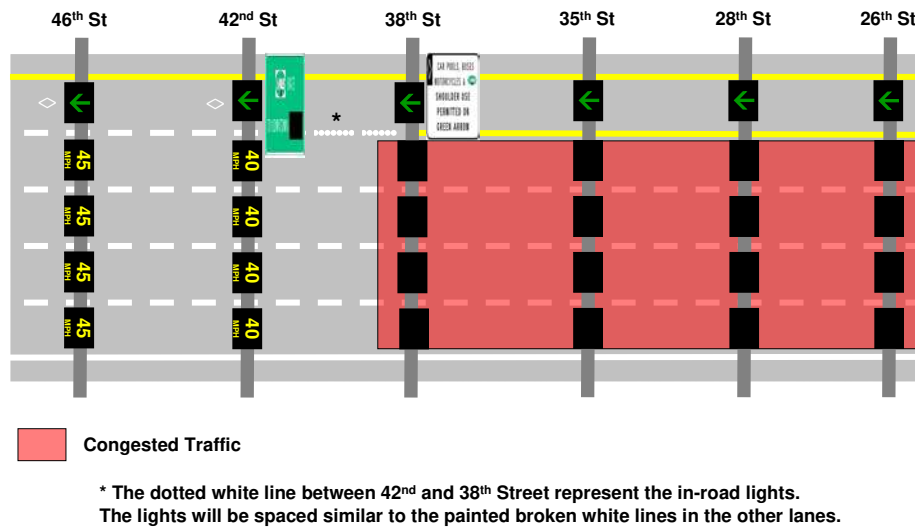
Figure MN-7. Striping and signing with PDSL open.
