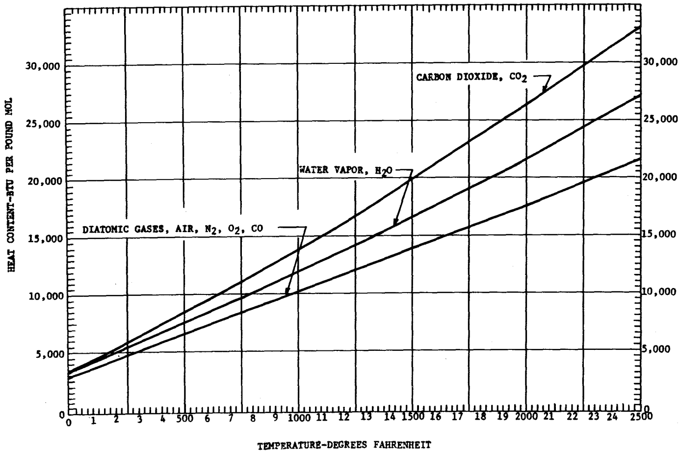
U. S. Army Corps of Engineers FIGURE A-2. CHART OF HEAT CONTENT OF GASES (CONSTANT PRESSURE)
