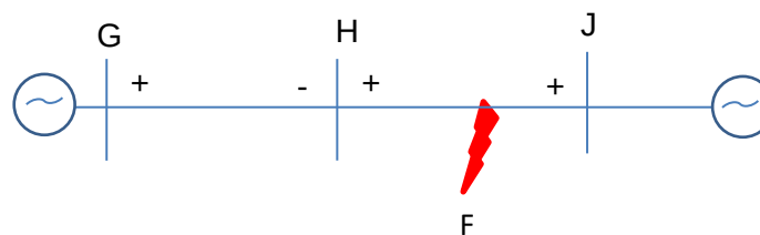
Figure 3. Current direction convention
