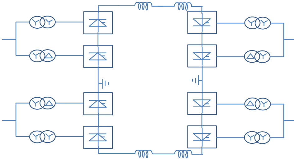
Figure 3. Bipolar HVDC configuration
