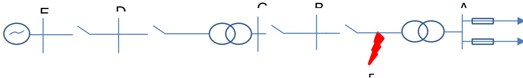
Figure 1. Radial electrical system with time discrimination
